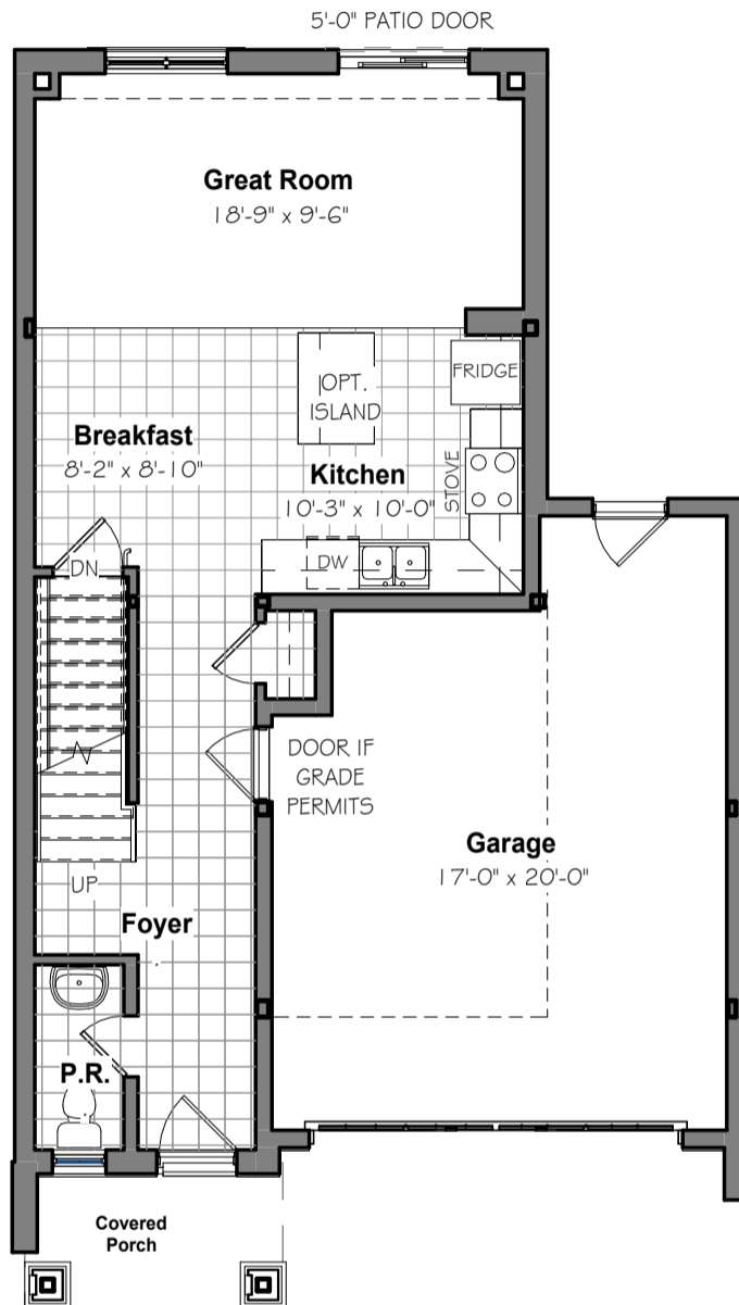
① Presentation Ground Floor 1/8" = 1'-0"
