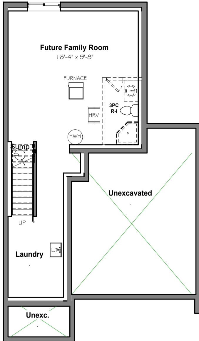
① Presentation Basement 1/8" = 1'-0"
